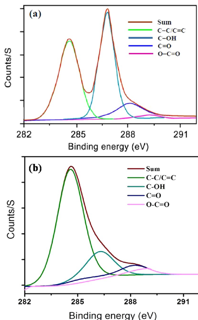
Figure 5. C1s XPS spectra of (a) graphene oxide and (b) dried RGO gel.
